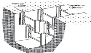
Vertical Aluminum Hydraulic Shoring (Stacked)
