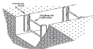
Vertical Aluminum Hydraulic Shoring (Spot Bracing)
