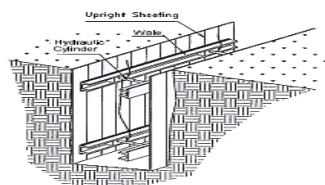
Aluminum Hydraulic Shoring Water System (Typical)
